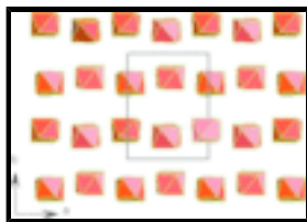
Fig. 2. : Projection of \text{EuO}_8 dodecahedra viewed along [0\ 0\ 1] direction.
