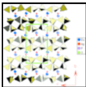
Fig. 1. : The structural arrangement of AgEu(PO_3)_4 along a axis.
